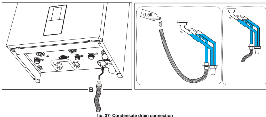
fig. 37- Condensate drain connection
