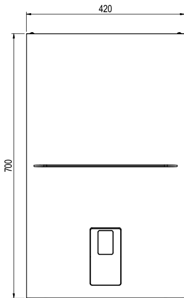
fig. 56- Front view
