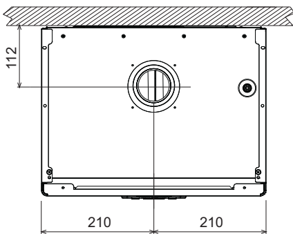
fig. 58- Top view
