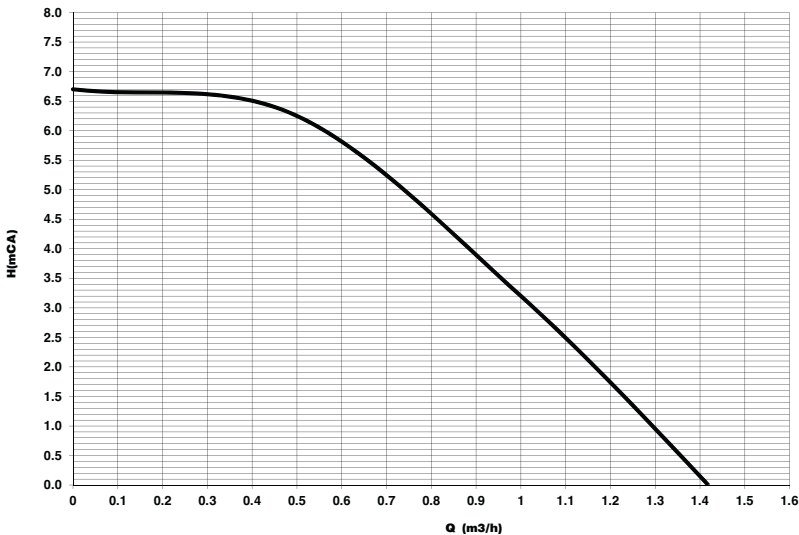
fig. 62- Residual head available for system
